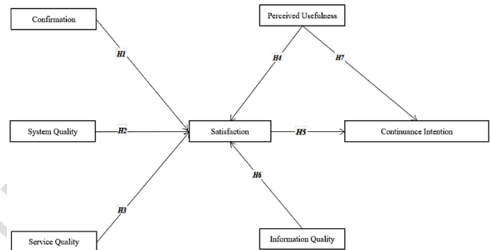
Figure 1: Conceptual Framework
